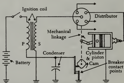
FIGURE 4-1. Battery ignition system.
